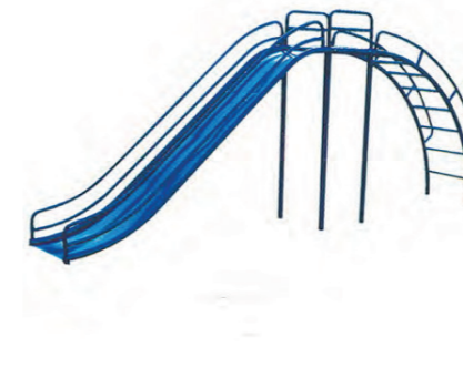
Modle No: LDK9005 Product Name: Children's Slide Size: 4350x500x2300mm
